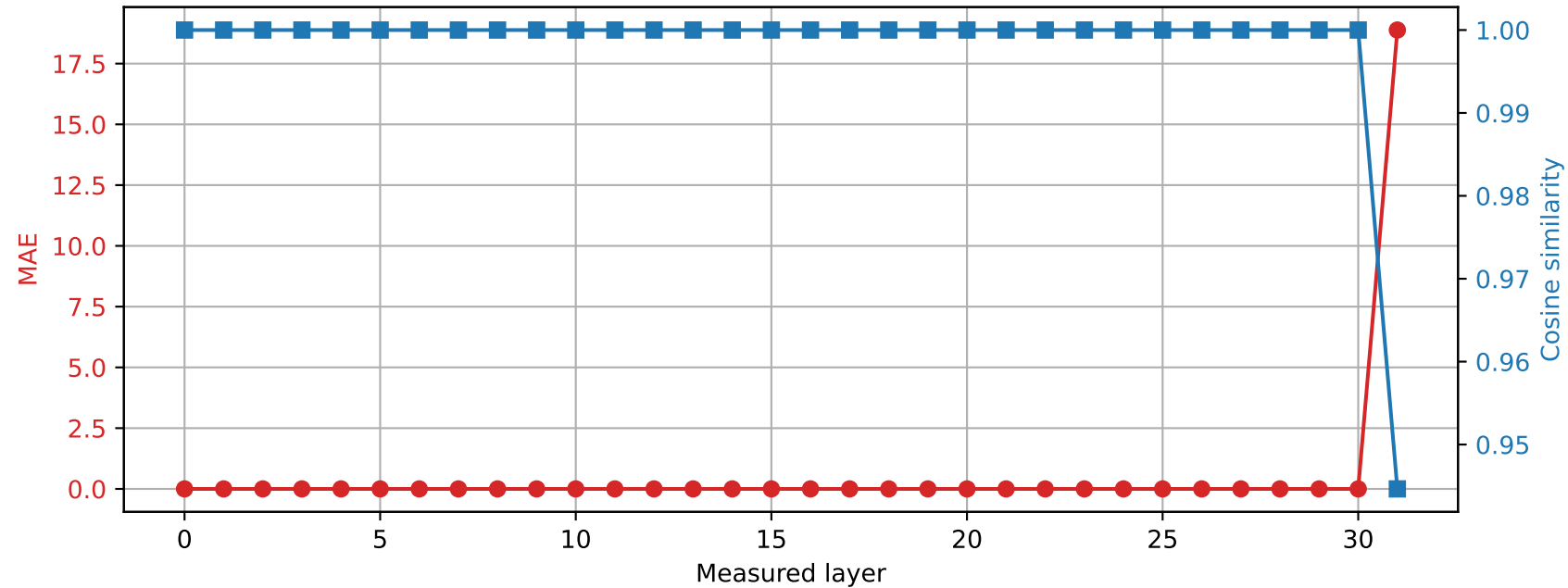
SmolLM2-360M | Prompt 3 Spared layer 30 | Hybrid vs quantized
