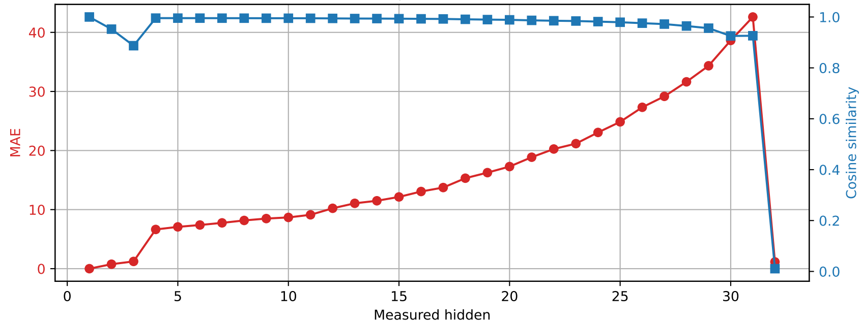
SmolLM2-360M | Prompt 4 Spared layer 0 | Unquantized vs hybrid
