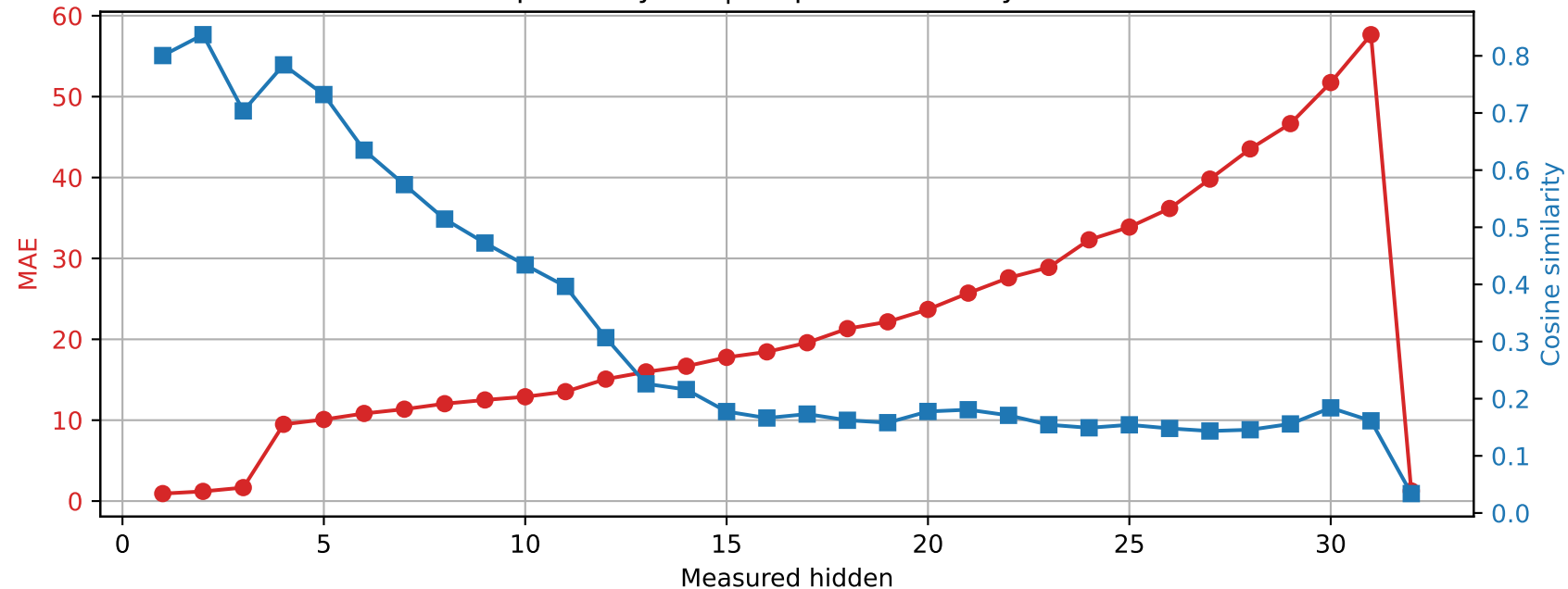
SmolLM2-360M | Prompt 4 Spared layer 1 | Unquantized vs hybrid
