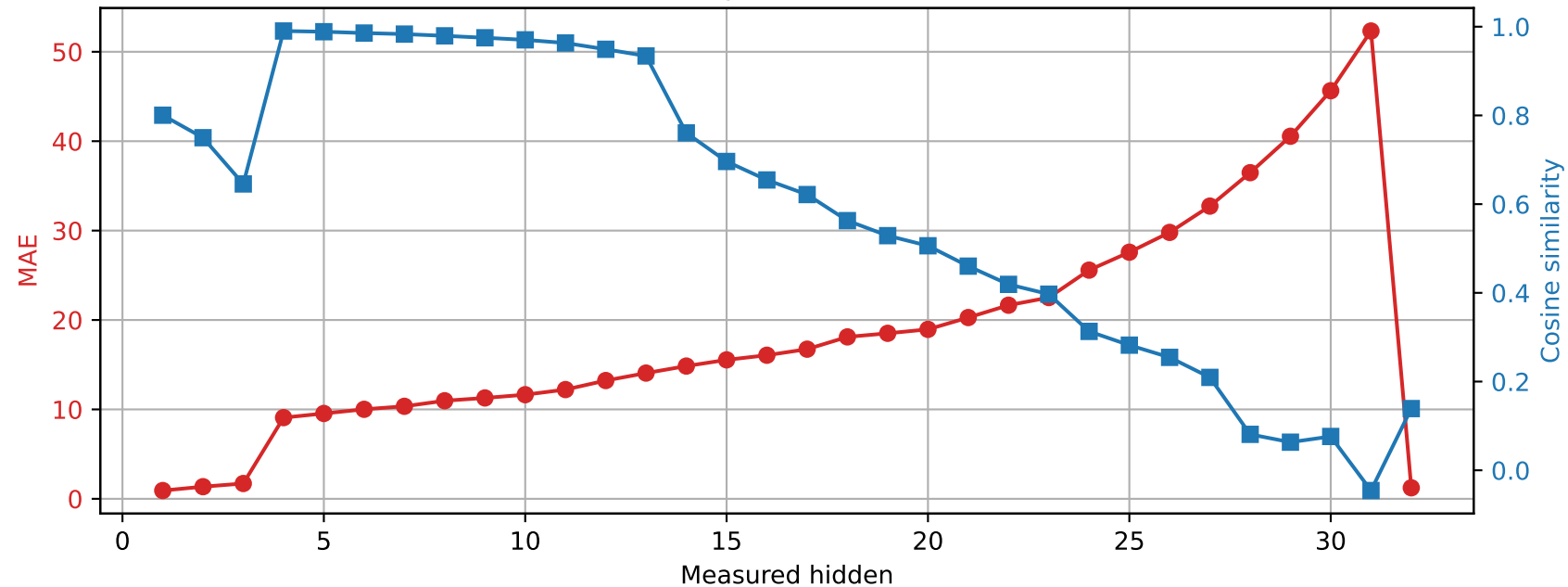
SmolLM2-360M | Prompt 4 Spared layer 2 | Unquantized vs hybrid
