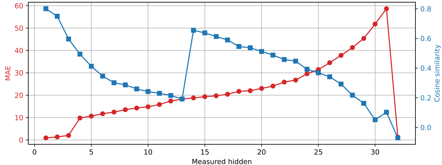
SmolLM2-360M | Prompt 4 Spared layer 4 | Unquantized vs hybrid
