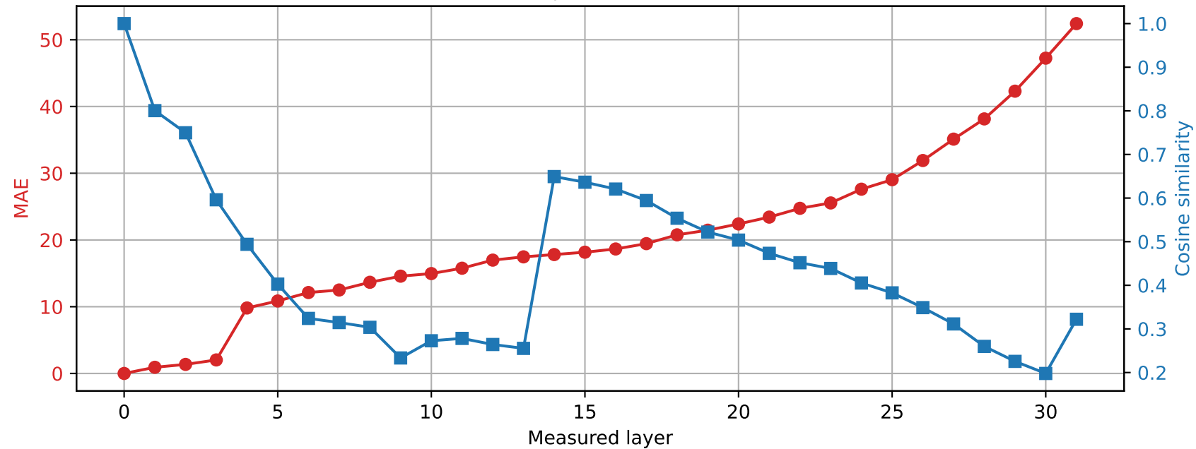
SmolLM2-360M | Prompt 4 Spared layer 6 | Hybrid vs unquantized
