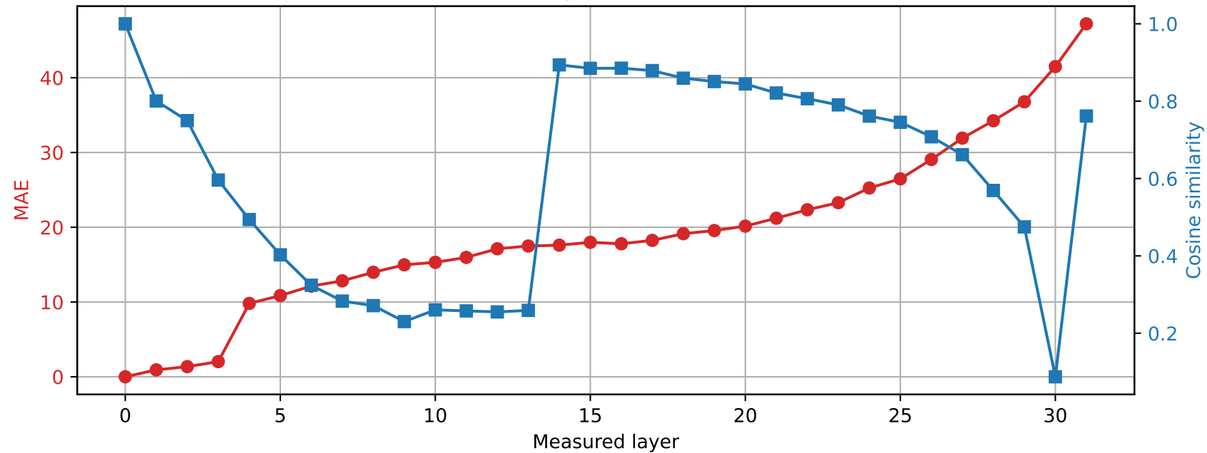
SmolLM2-360M | Prompt 4 Spared layer 15 | Hybrid vs unquantized
