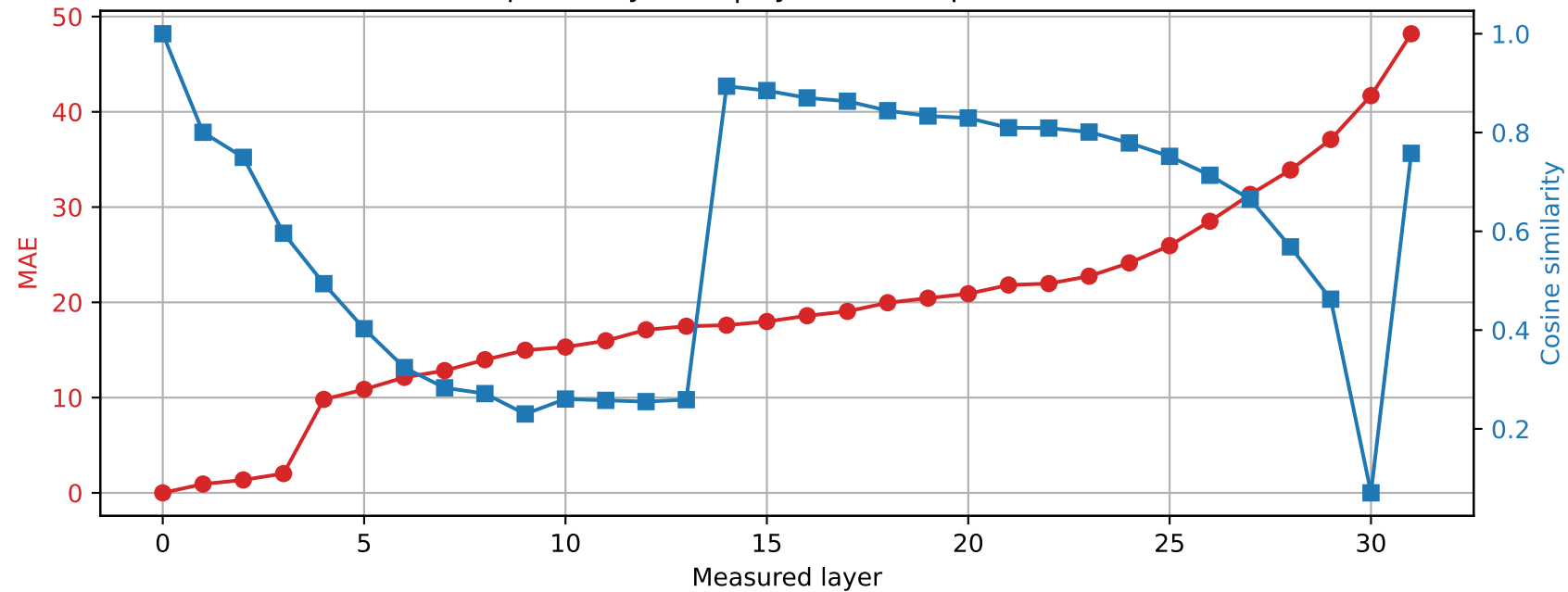
SmolLM2-360M | Prompt 4 Spared layer 21 | Hybrid vs unquantized
