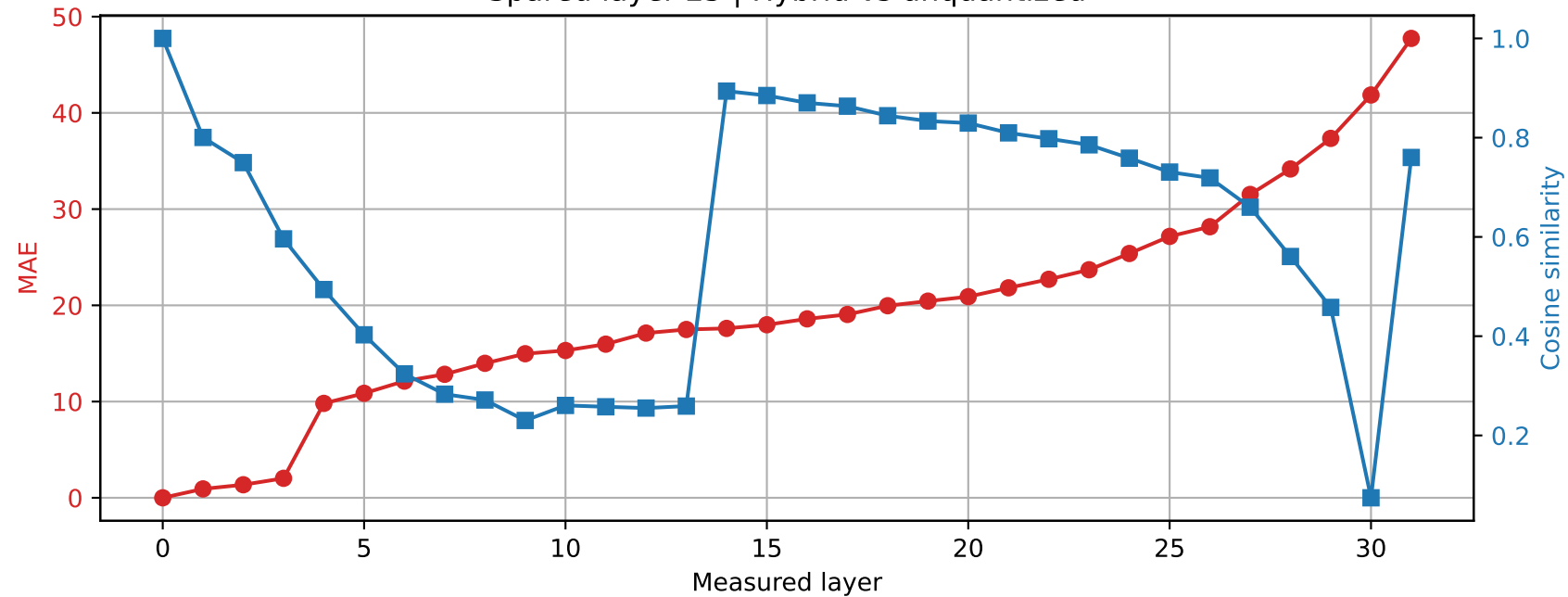
SmolLM2-360M | Prompt 4 Spared layer 25 | Hybrid vs unquantized
