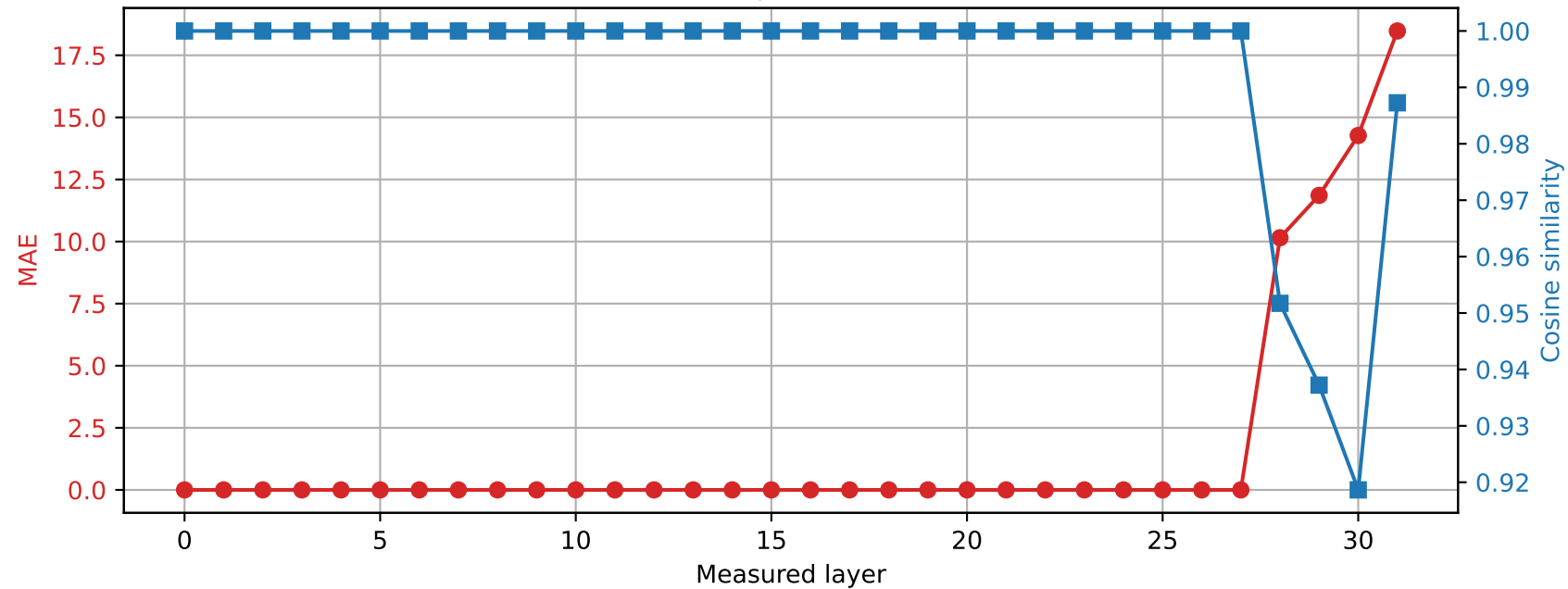
SmolLM2-360M | Prompt 4 Spared layer 27 | Hybrid vs quantized
