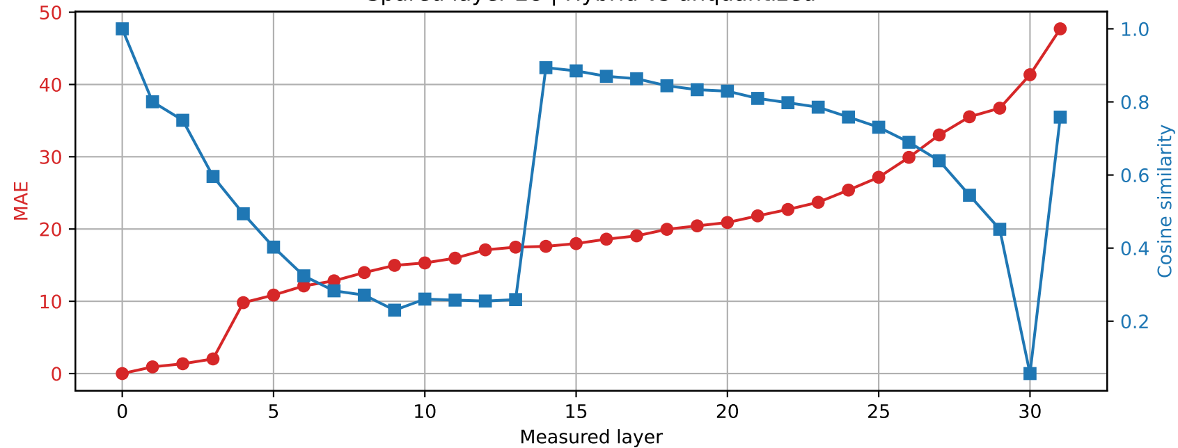
SmolLM2-360M | Prompt 4 Spared layer 28 | Hybrid vs unquantized
