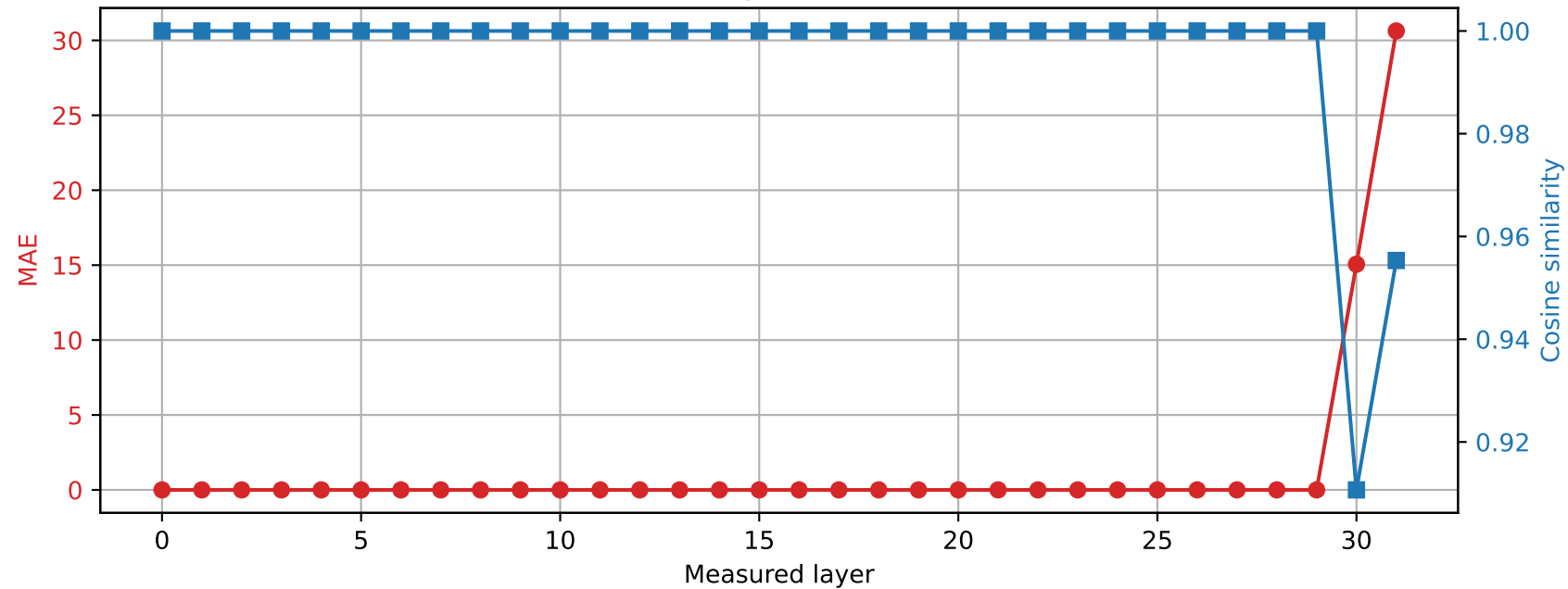
SmolLM2-360M | Prompt 4 Spared layer 29 | Hybrid vs quantized
