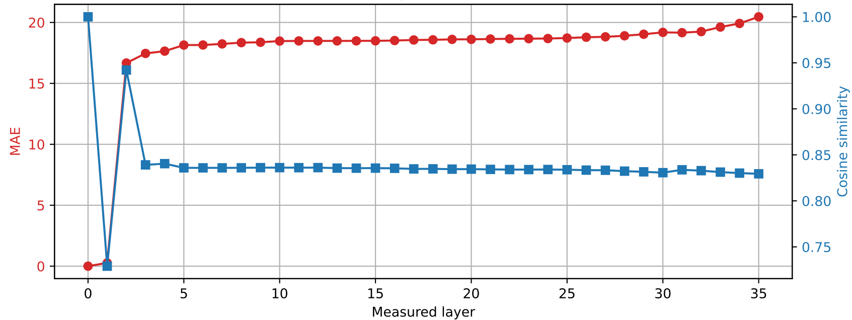
Qwen2.5-3B | Prompt 0 Spared layer 0 | Hybrid vs quantized
