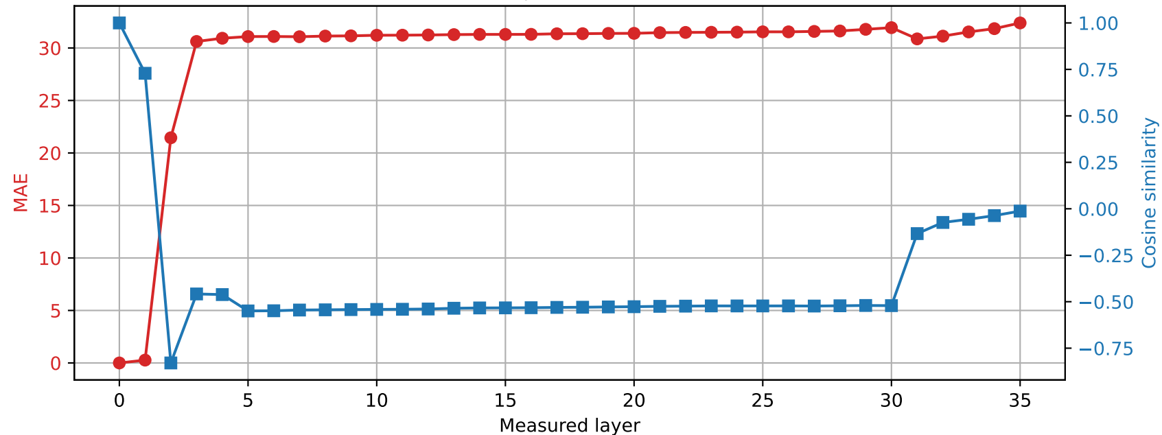
Qwen2.5-3B | Prompt 0 Spared layer 6 | Hybrid vs unquantized
