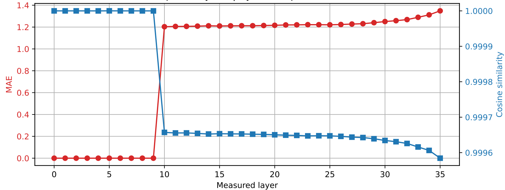
Qwen2.5-3B | Prompt 0 Spared layer 9 | Hybrid vs quantized
