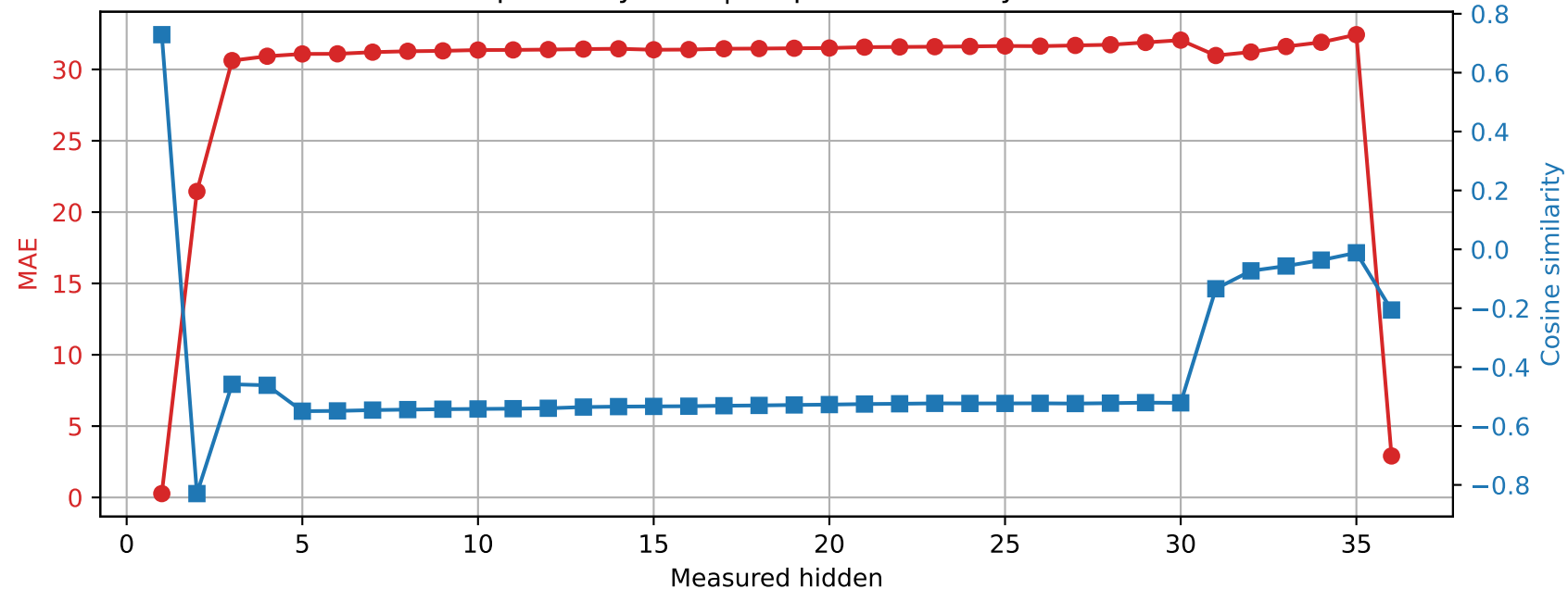
Qwen2.5-3B | Prompt 0 Spared layer 14 | Unquantized vs hybrid
