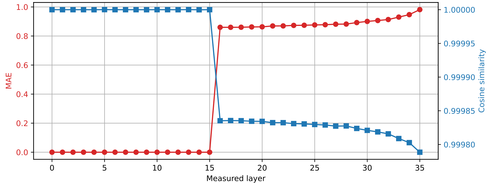
Qwen2.5-3B | Prompt 0 Spared layer 15 | Hybrid vs quantized
