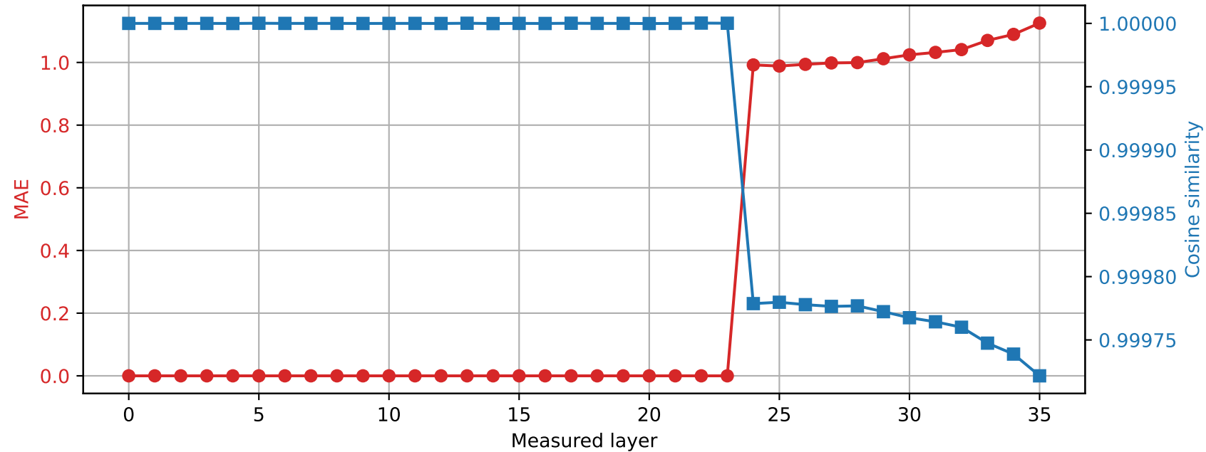
Qwen2.5-3B | Prompt 0 Spared layer 23 | Hybrid vs quantized
