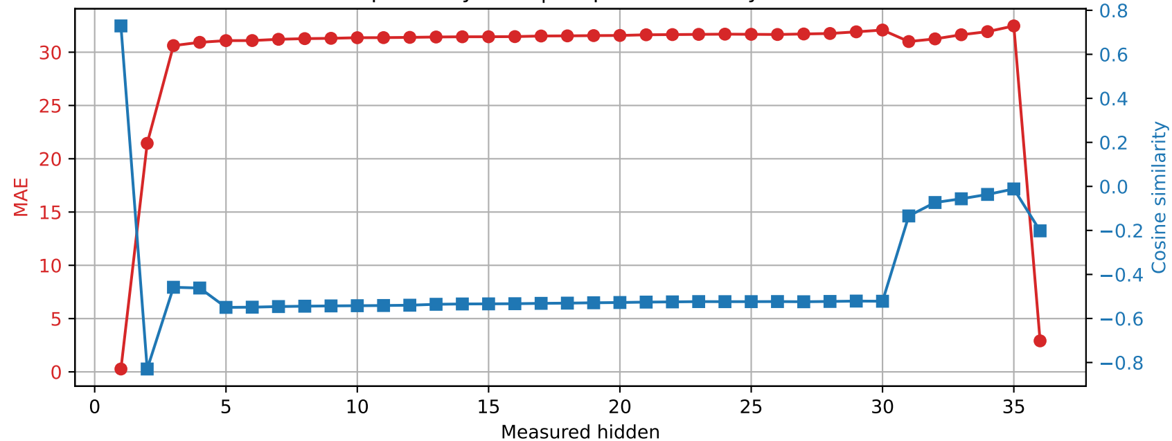
Qwen2.5-3B | Prompt 0 Spared layer 24 | Unquantized vs hybrid
