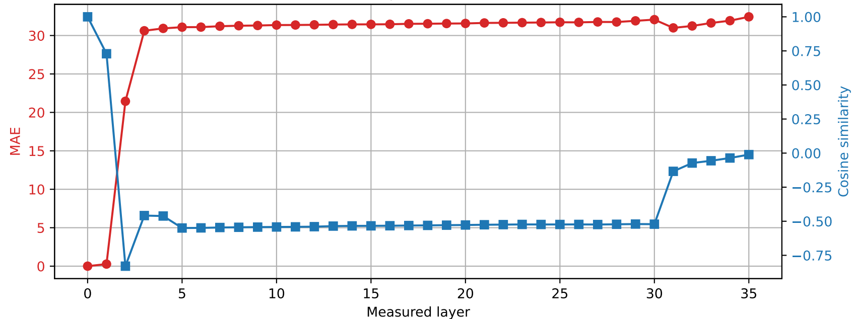
Qwen2.5-3B | Prompt 0 Spared layer 27 | Hybrid vs unquantized
