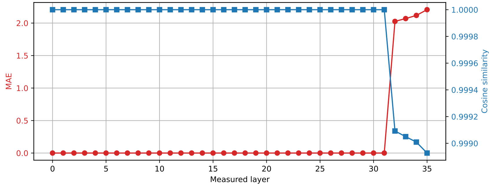
Qwen2.5-3B | Prompt 0 Spared layer 31 | Hybrid vs quantized
