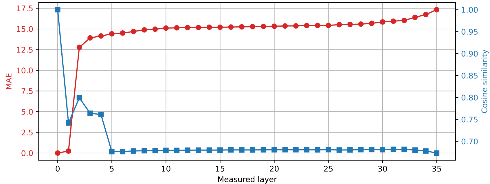
Qwen2.5-3B | Prompt 1 Spared layer 0 | Hybrid vs quantized
