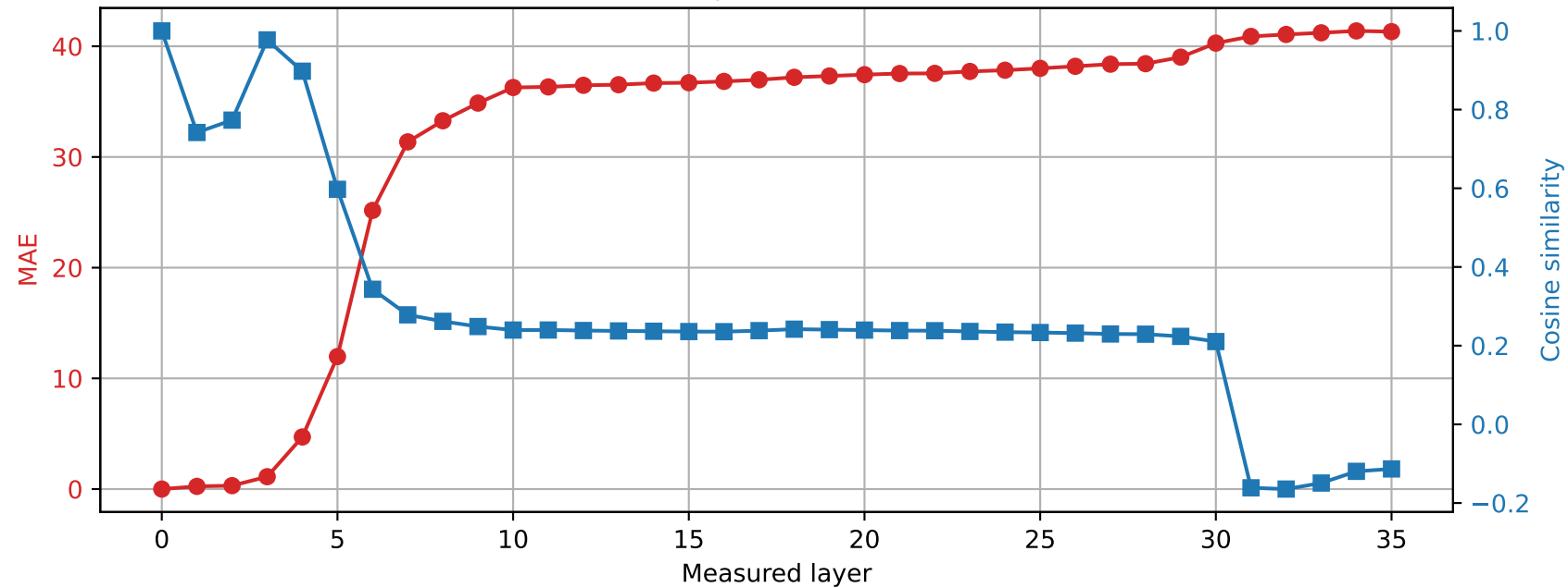
Qwen2.5-3B | Prompt 1 Spared layer 1 | Hybrid vs unquantized
