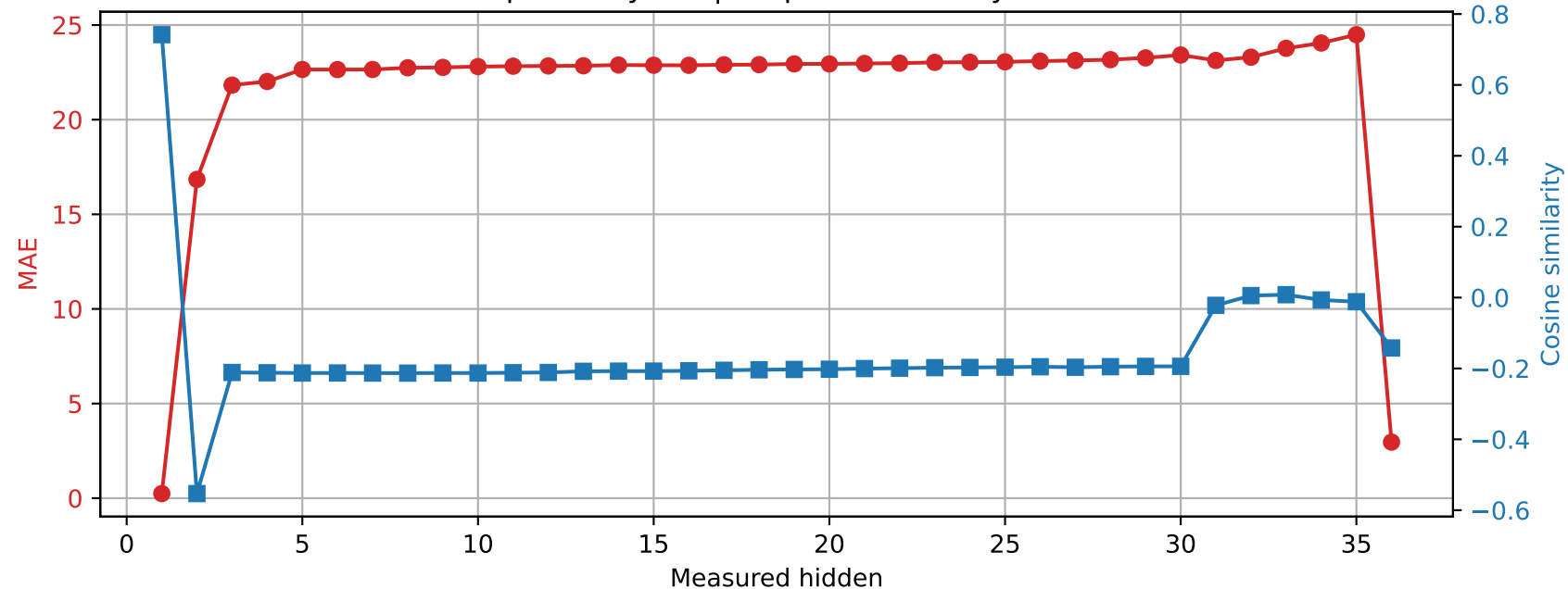
Qwen2.5-3B | Prompt 1 Spared layer 4 | Unquantized vs hybrid
