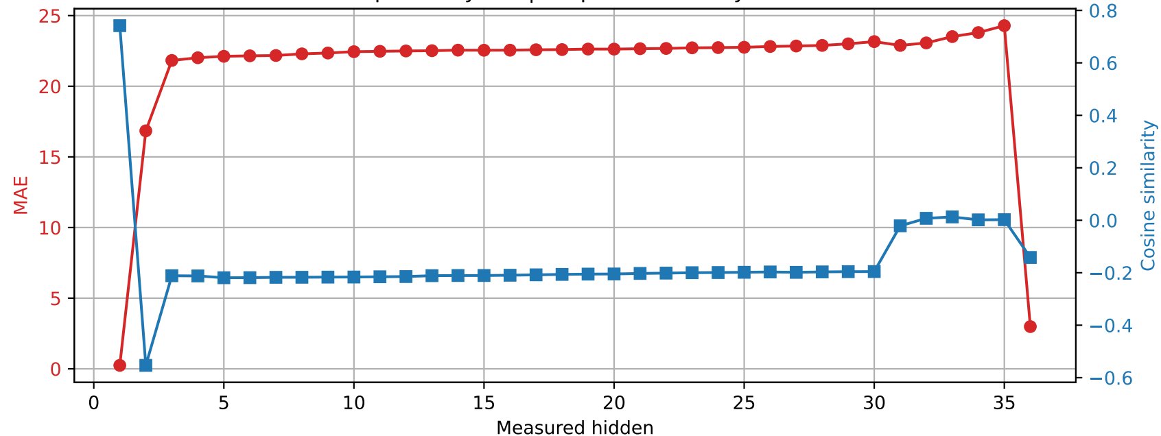
Qwen2.5-3B | Prompt 1 Spared layer 6 | Unquantized vs hybrid
