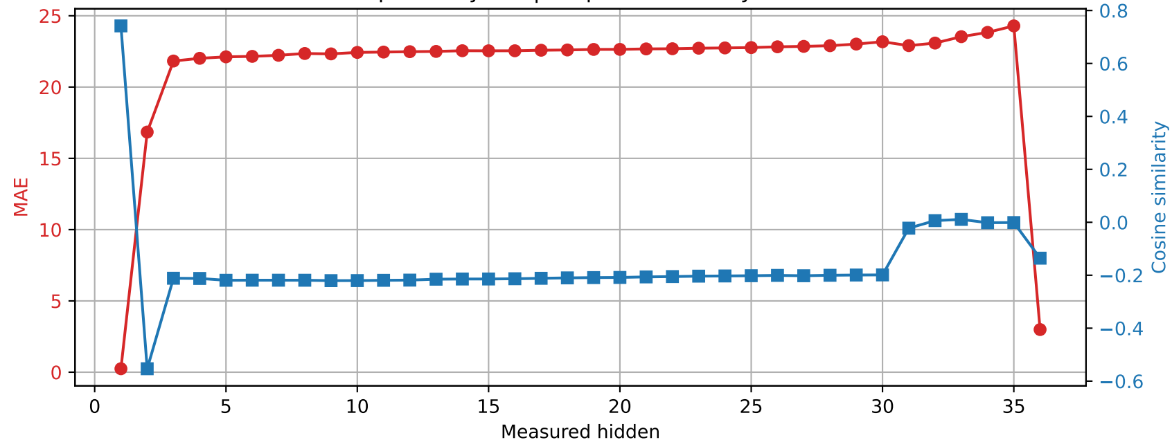
Qwen2.5-3B | Prompt 1 Spared layer 8 | Unquantized vs hybrid
