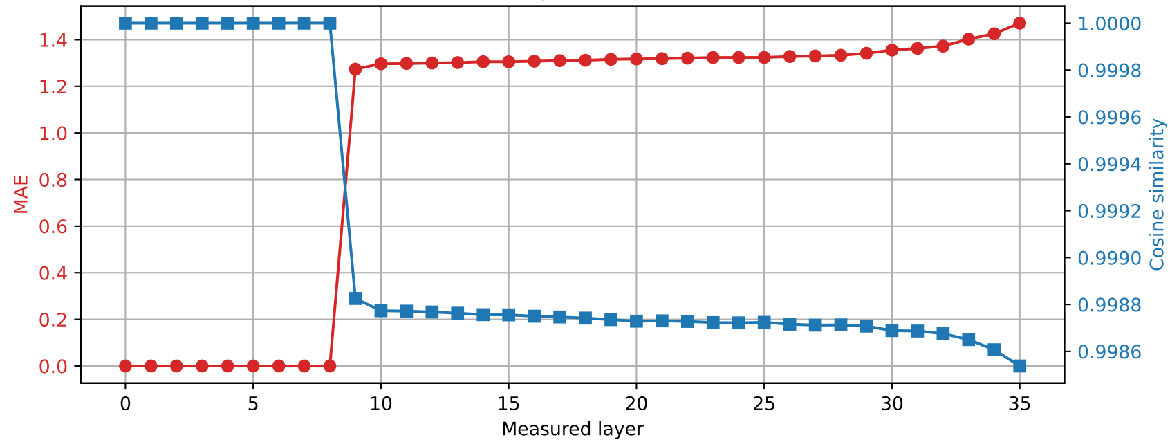
Qwen2.5-3B | Prompt 1 Spared layer 8 | Hybrid vs quantized
