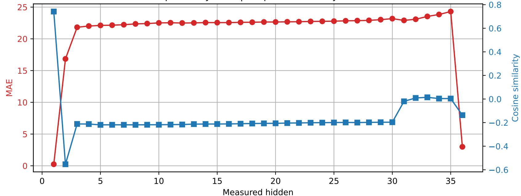
Qwen2.5-3B | Prompt 1 Spared layer 11 | Unquantized vs hybrid
