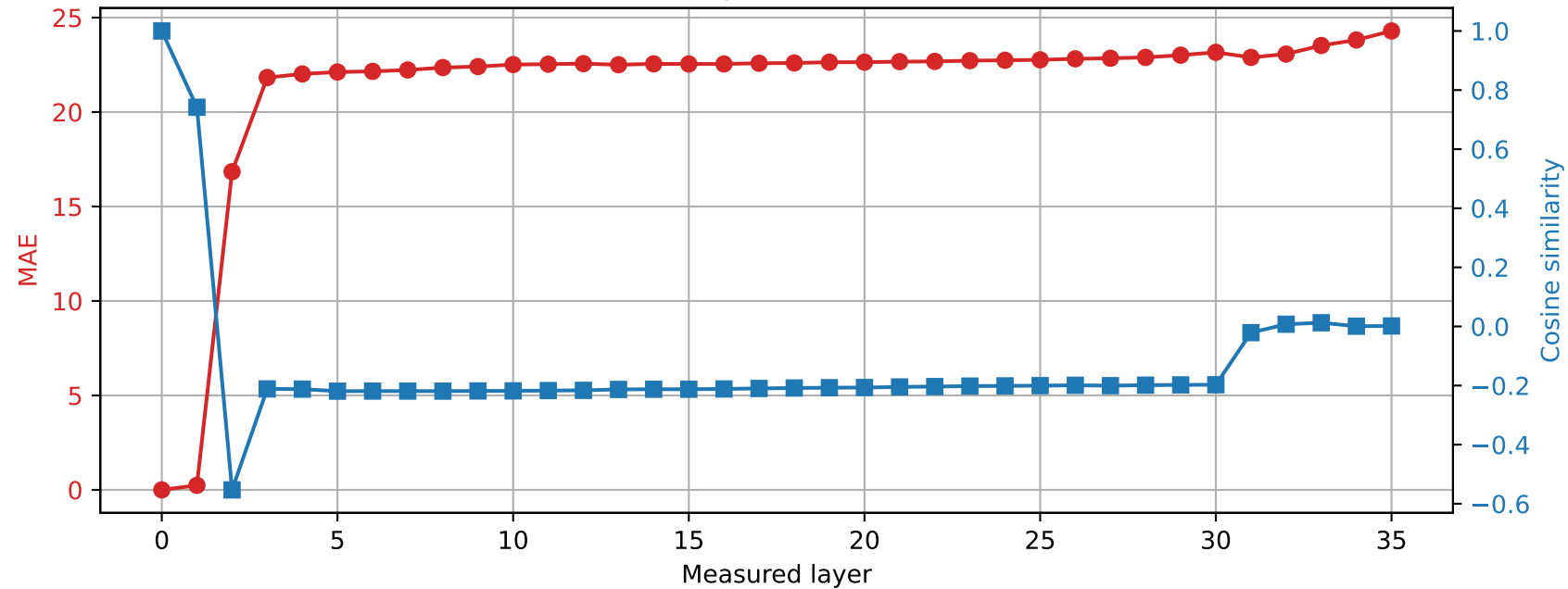
Qwen2.5-3B | Prompt 1 Spared layer 12 | Hybrid vs unquantized
