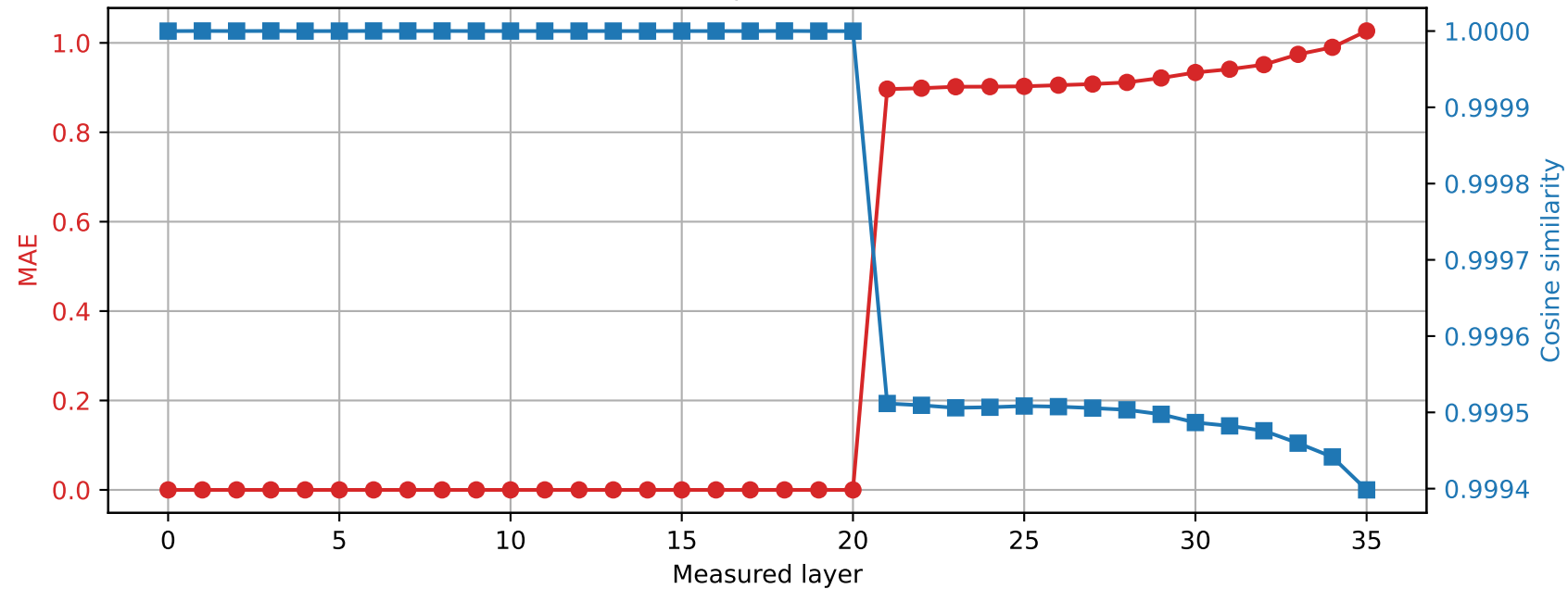
Qwen2.5-3B | Prompt 1 Spared layer 20 | Hybrid vs quantized
