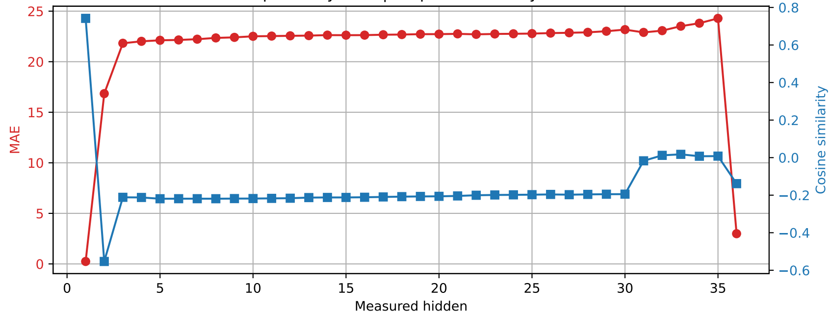
Qwen2.5-3B | Prompt 1 Spared layer 21 | Unquantized vs hybrid
