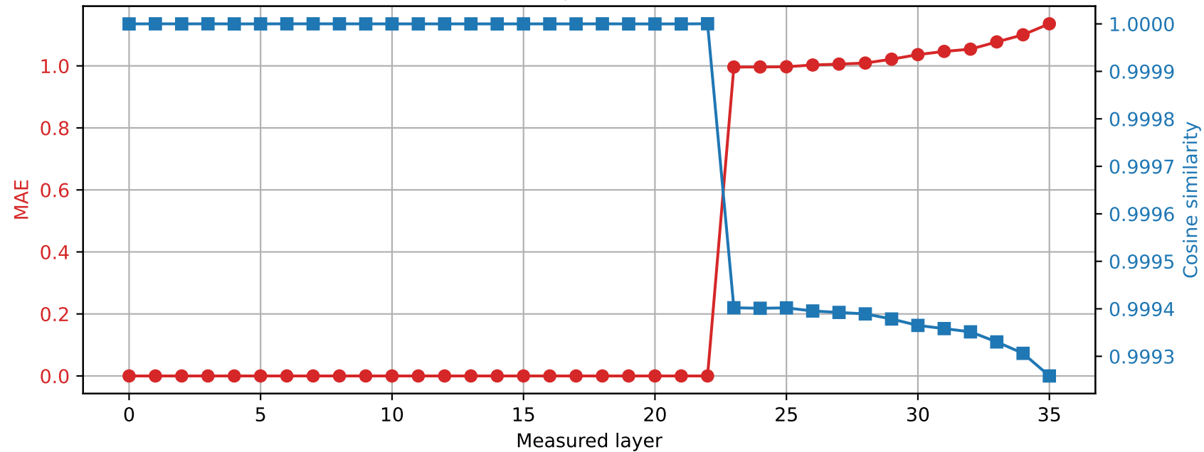
Qwen2.5-3B | Prompt 1 Spared layer 22 | Hybrid vs quantized
