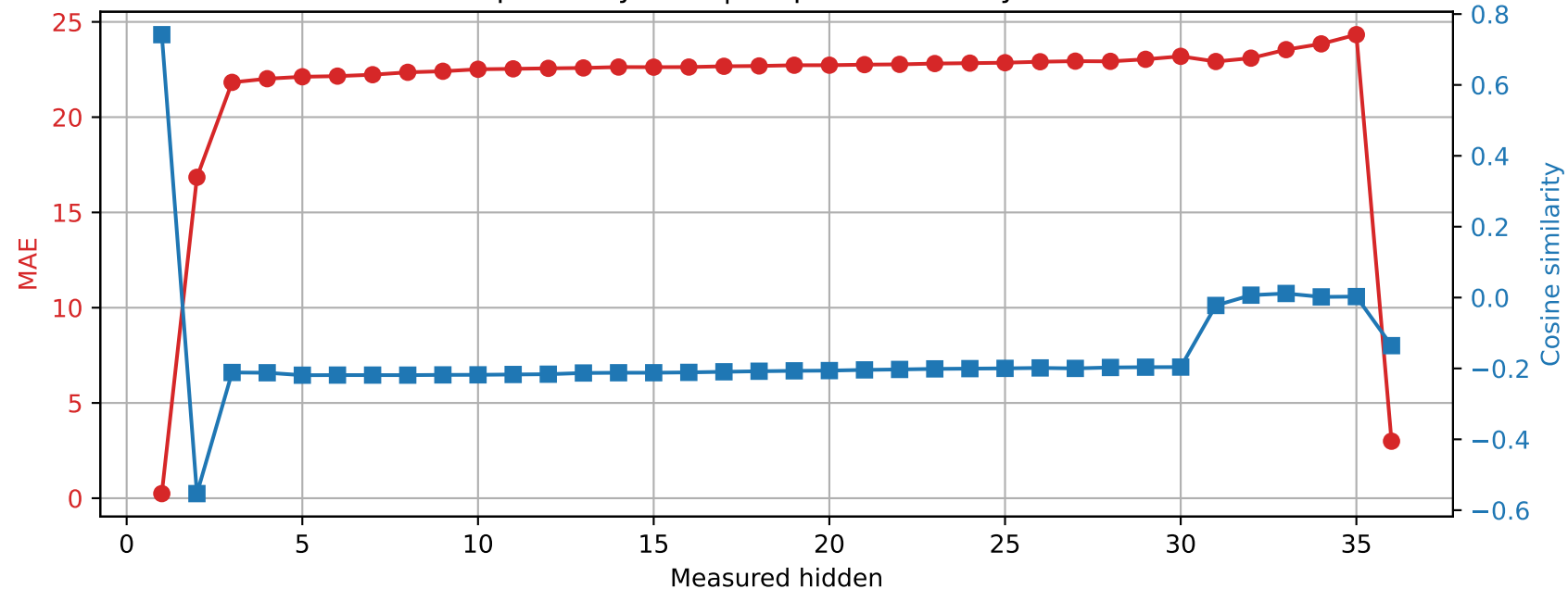
Qwen2.5-3B | Prompt 1 Spared layer 27 | Unquantized vs hybrid
