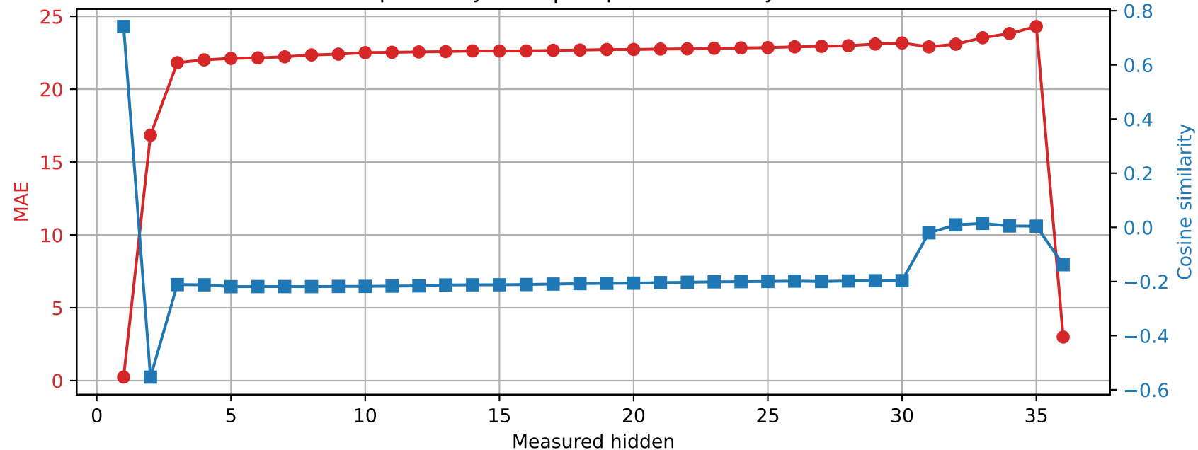
Qwen2.5-3B | Prompt 1 Spared layer 29 | Unquantized vs hybrid
