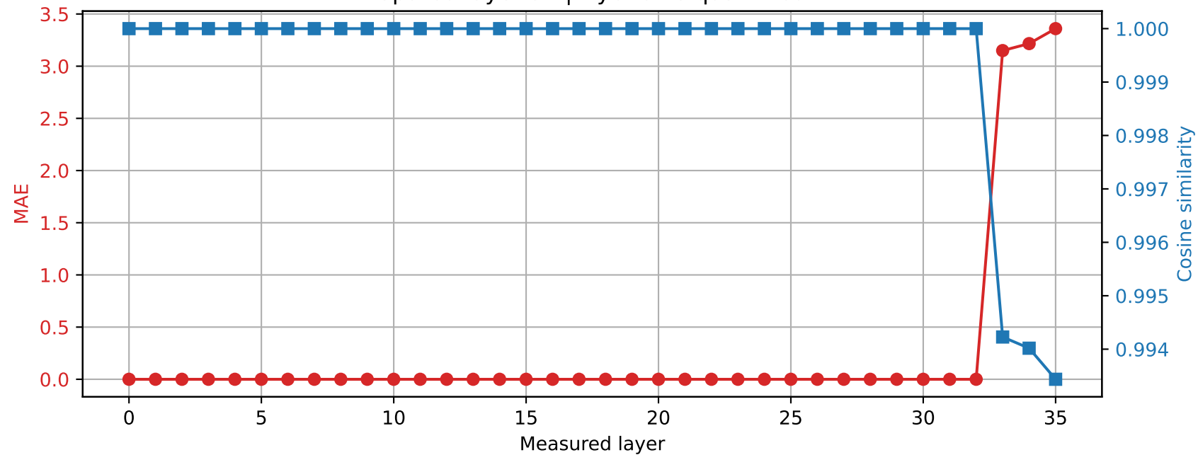
Qwen2.5-3B | Prompt 1 Spared layer 32 | Hybrid vs quantized
