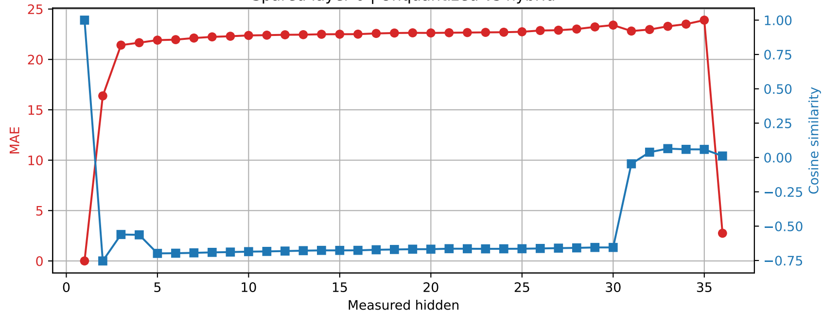
Qwen2.5-3B | Prompt 2 Spared layer 0 | Unquantized vs hybrid
