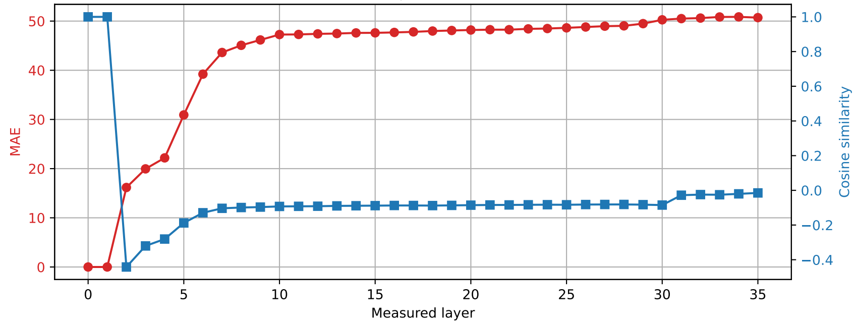
Qwen2.5-3B | Prompt 2 Spared layer 1 | Hybrid vs quantized
