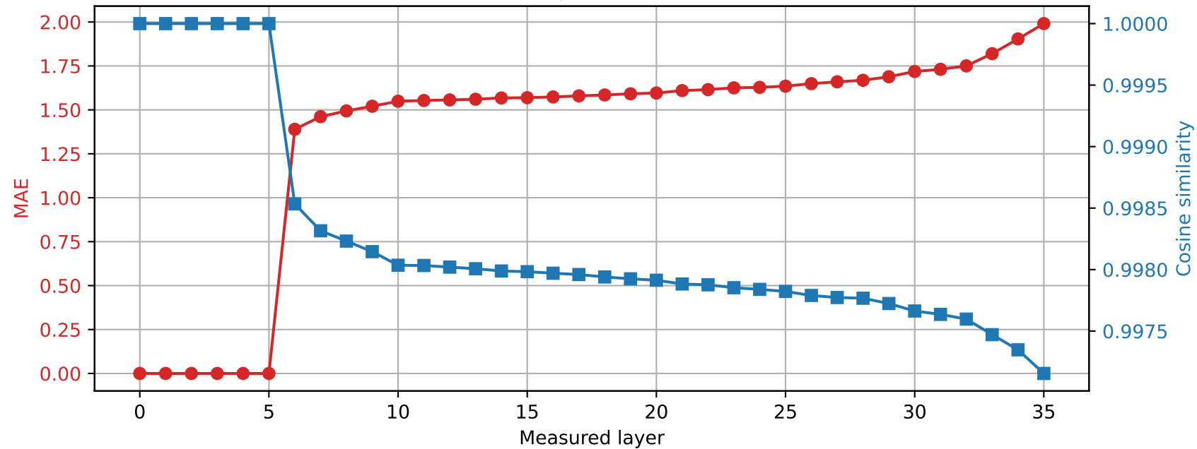
Qwen2.5-3B | Prompt 2 Spared layer 5 | Hybrid vs quantized
