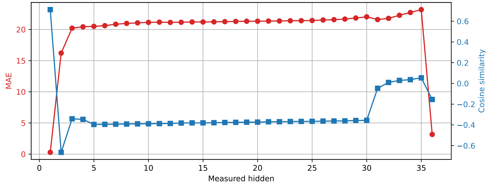
Qwen2.5-3B | Prompt 2 Spared layer 11 | Unquantized vs hybrid
