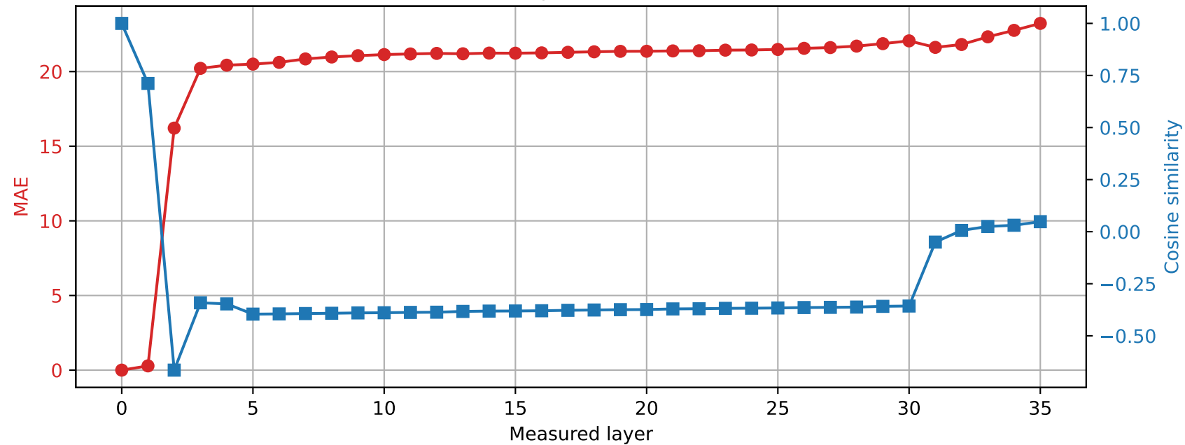
Qwen2.5-3B | Prompt 2 Spared layer 12 | Hybrid vs unquantized
