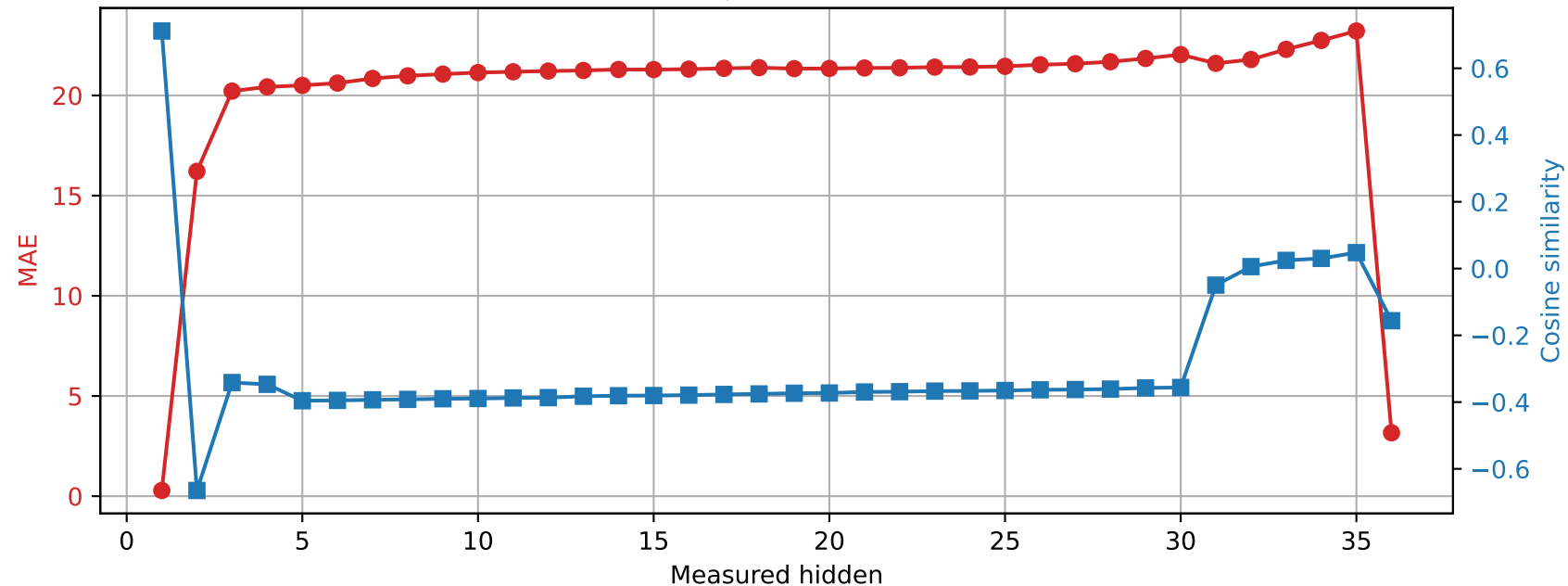
Qwen2.5-3B | Prompt 2 Spared layer 18 | Unquantized vs hybrid
