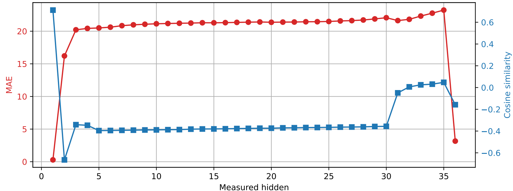
Qwen2.5-3B | Prompt 2 Spared layer 19 | Unquantized vs hybrid
