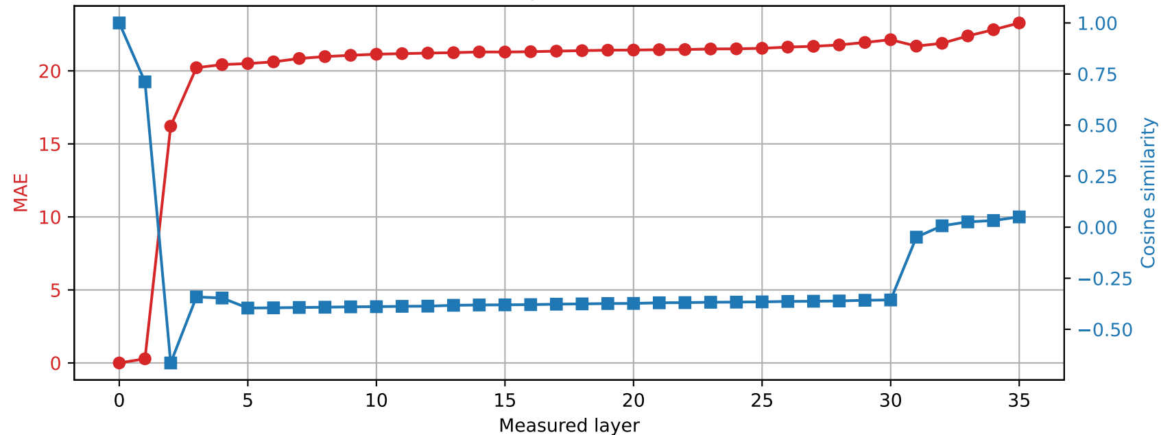
Qwen2.5-3B | Prompt 2 Spared layer 35 | Hybrid vs unquantized
