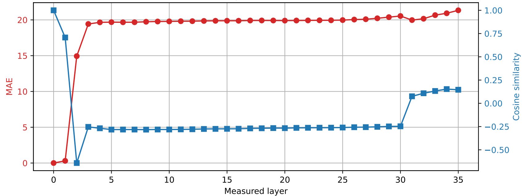
Qwen2.5-3B | Prompt 3 Spared layer 3 | Hybrid vs unquantized
