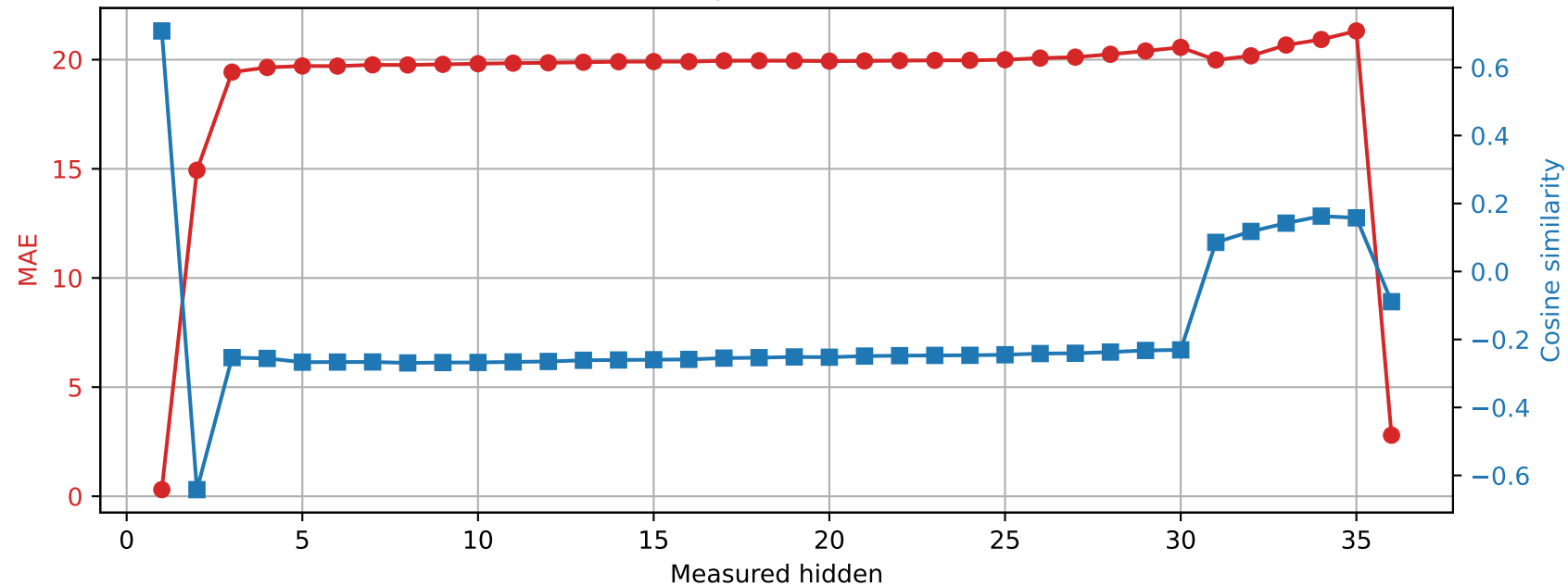
Qwen2.5-3B | Prompt 3 Spared layer 7 | Unquantized vs hybrid
