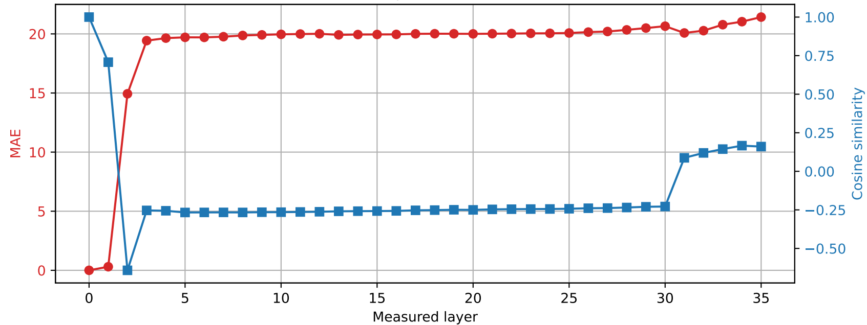
Qwen2.5-3B | Prompt 3 Spared layer 12 | Hybrid vs unquantized
