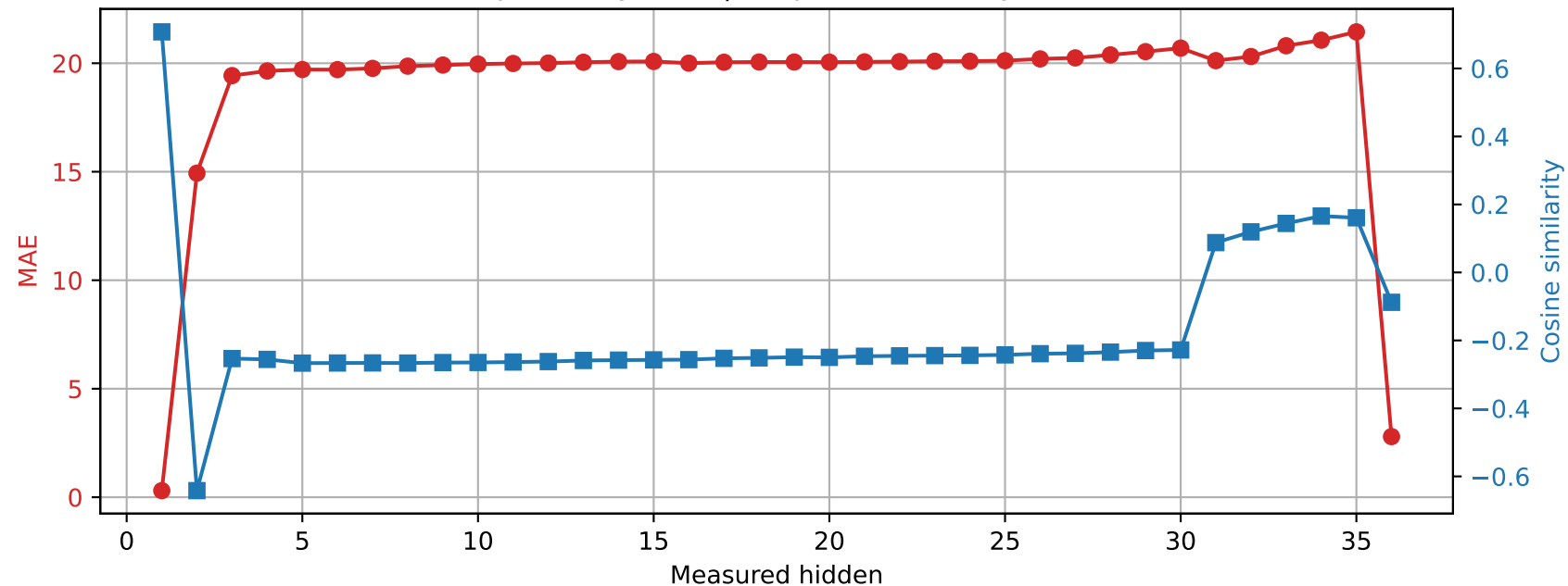
Qwen2.5-3B | Prompt 3 Spared layer 15 | Unquantized vs hybrid
