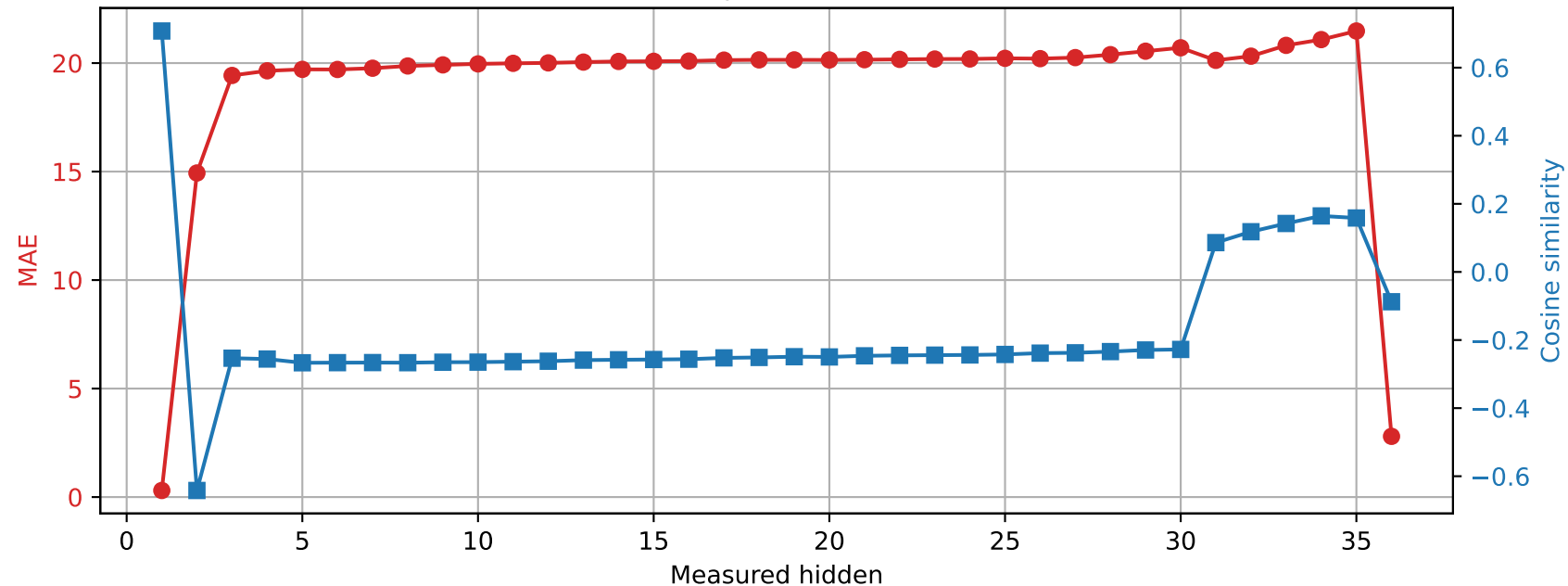
Qwen2.5-3B | Prompt 3 Spared layer 25 | Unquantized vs hybrid
