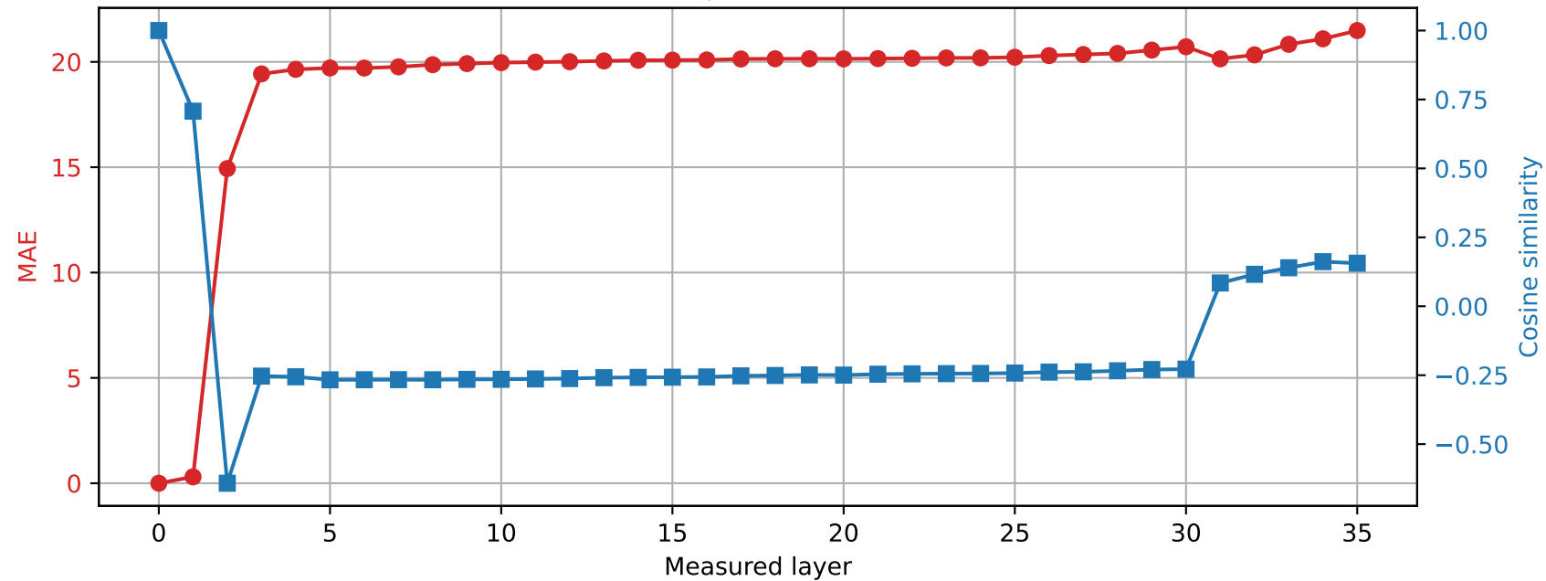
Qwen2.5-3B | Prompt 3 Spared layer 27 | Hybrid vs unquantized
