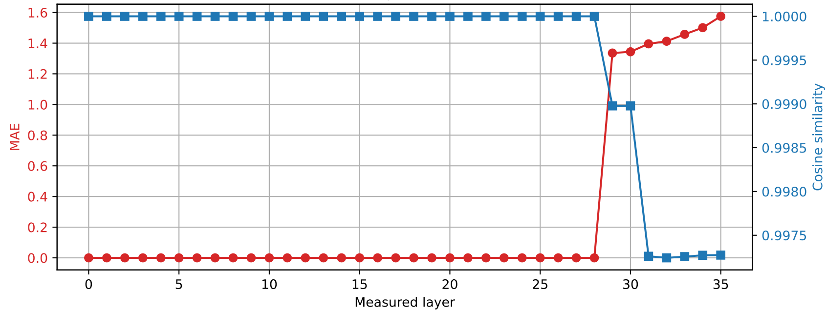
Qwen2.5-3B | Prompt 3 Spared layer 28 | Hybrid vs quantized
